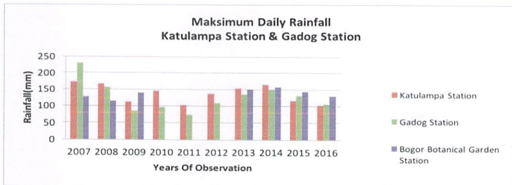
Figure 3. Maximum Rainfall Data in three (3) Stations Observations
